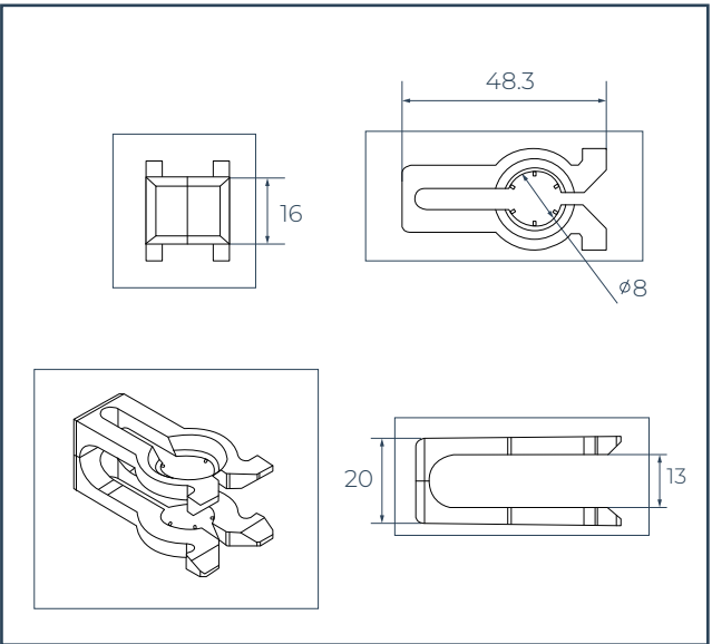
Mini Size (Suitable for 8-12mm rebar)
