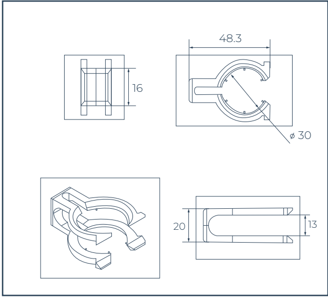
Large Size (Suitable for 30-35mm rebar)
