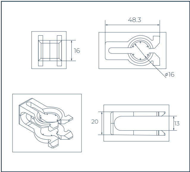
Standard Size (Suitable for 16-20mm rebar)
